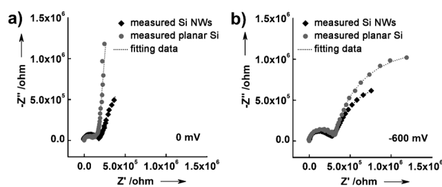
Figure 3. Nyquist plots at 0 \text{ V} (a) and -0.600 \text{ V} (b) for SiNWs (black) and planar Si (gray). The dotted lines are fitted to the data.
